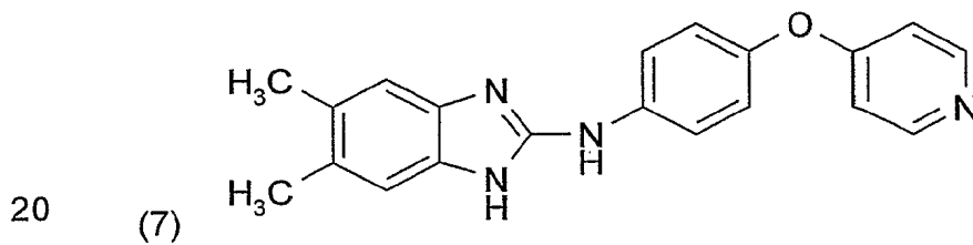
(5,6-Dimethyl-1H-benzimidazol-2-yl)-[4-(pyridin-4-yloxy)-phenyl]-amin
